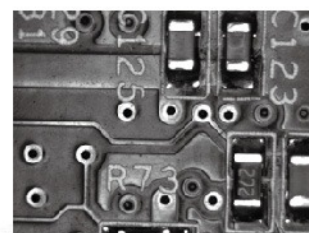
GL-DO5411W PC Board
